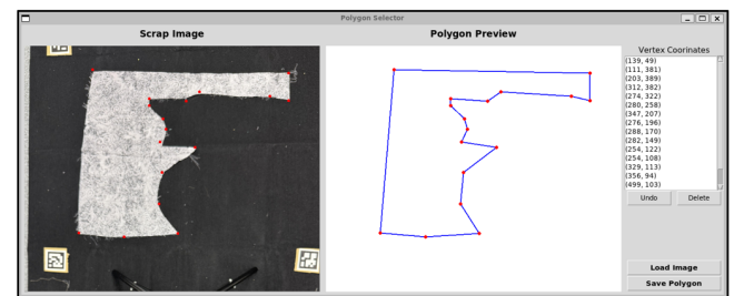
Figure 3: The segmentation interface for converting each scrap into a digital form. It allows users to manually specify the desired region of each photographed scrap by outlining it as a polygon, which is then imported into the system.
